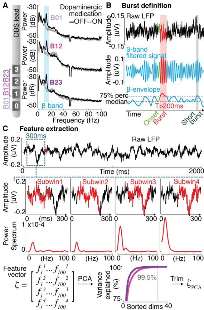
Figure 1. (A) Comparison of power spectrum profiles of LFPs recorded as bipolar signals from consecutive pairs of electrodes from a DBS lead for patient S1, either 'ON' dopaminergic medication (gray traces) or 'OFF' (black). The beta band is derived as \pm 3 Hz around the peak distinguishing both conditions (cyan). (B) Definition of beta bursts: The envelope of the beta signal is thresholded at the 75% percentile amplitude. Only bursts of durations exceeding 200ms are defined as pathological. (C) Parameterisation: For each sample (every 50ms), frequency components are calculated over a window of 300ms. The feature vector is composed of spectral values over moving subwindows (175ms, 75% overlap). PCA is applied to reduce the dimensionality (99.5% of the variance).
