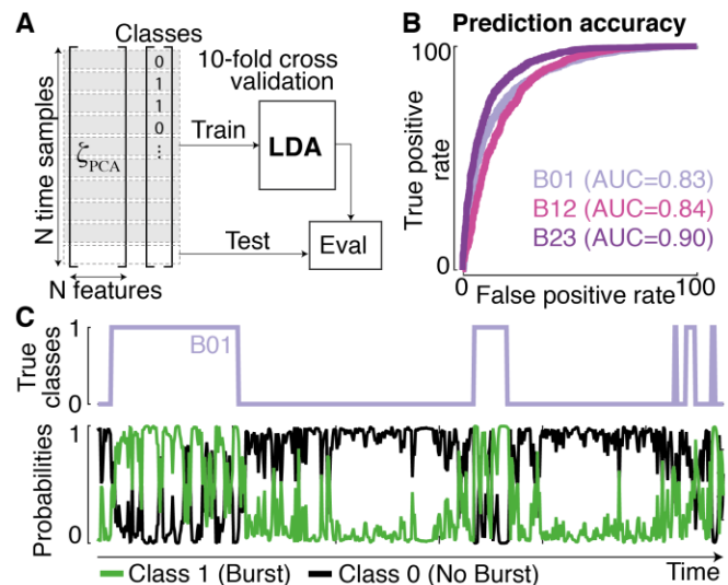
Figure 2. (A) Classification methodology. Feature vector comprising frequency changes preceding each time sample and binarized classes (burst vs. no burst) are employed to train and test an LDA classifier. Accuracy is validated using 10-fold cross-validation. (B) ROC curves for each pair of bilateral electrodes for subject S1. (C) Example traces of true class definition for one contact pair and prediction probabilities for each class.
